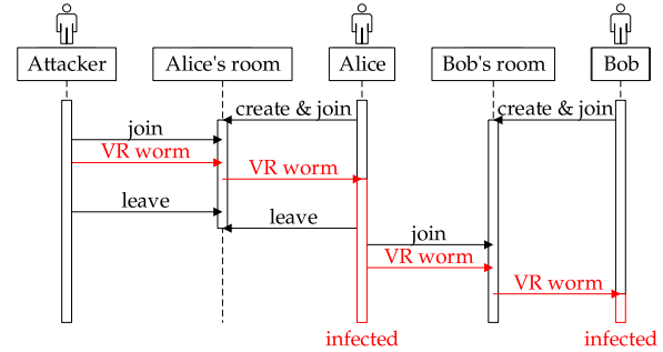
Fig. 10. Sequence diagram of initial VR worm infection (in Alice's room) and propagation from one user to another when they meet in VR room (in Bob's room).
