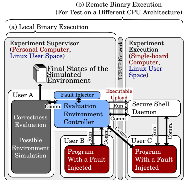
Figure 2: The architecture of the Evaluation Environment for execution and testing of programs running (a) on the same computer as the Evaluation Environment; (b) remotely on another computer utilizing (possibly) different architecture.
