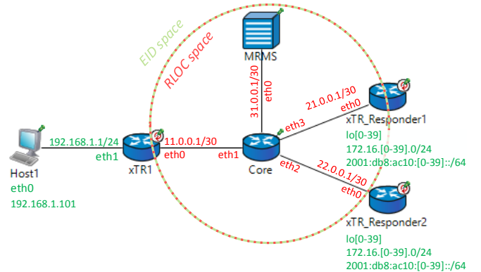
Figure 19. LISP testing topology for merged RLOC probing
