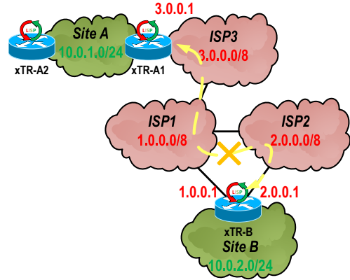
Figure 7. Locator Path Liveness Problem illustration
