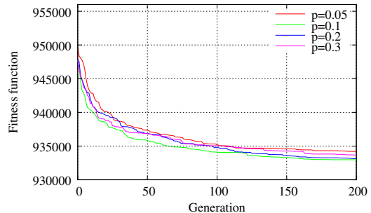
Figure 4: Evolution for Opt_1 and O_{mut} with p_{mut} = 0.05, 0.1, 0.2, 0.3 (average from ten runs).
