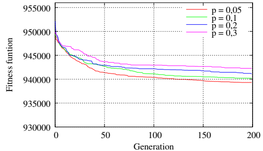
Figure 3: Evolution for Opt_1 and O_{mut} with p_{mut}(u) = 0.05, 0.1, 0.2, 0.3 (average from ten runs).
