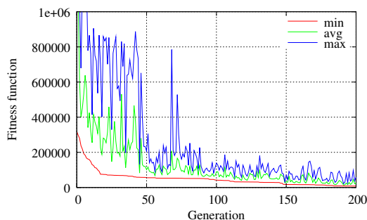
Figure 7: Evolution for Opt_1 and O_{mut} with p_{mut} = 0.15 (average from ten runs).
