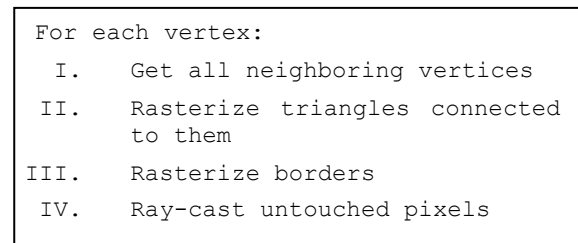
Figure 2. Rasterization algorithm
