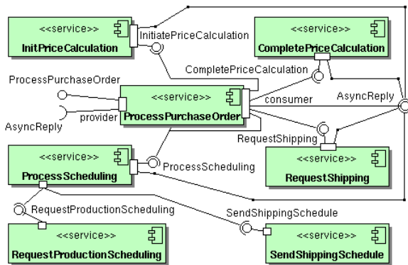
Figure 2: An overview of identified services, their interfaces and connections.
