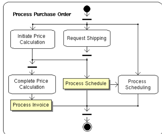
Figure 5: Behaviour of service ProcessPurchaseOrder in the context of used services and internal processes.
