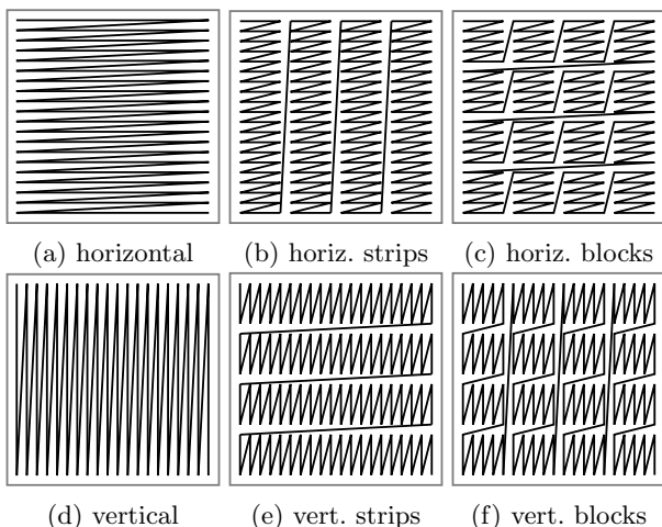
Fig. 7: Processing orders evaluated with both cores (vertical and diagonal).
