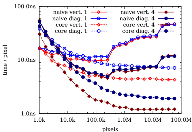
Fig. 21: Comparison of the parallelized naive and the parallelized core approaches on AMD CPU.
