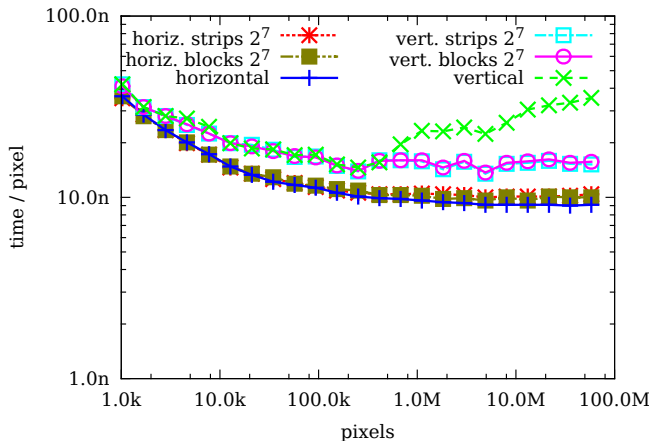
Fig. 11: Evaluation of processing orders. Diagonal core on AMD platform.
