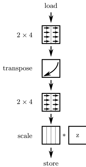
Fig. 13: 4 \times 4 vertical core. In 2 \times 4 blocks, all operations of the vertical vectorization are performed over SSE vector registers instead of ordinary scalar ones.
