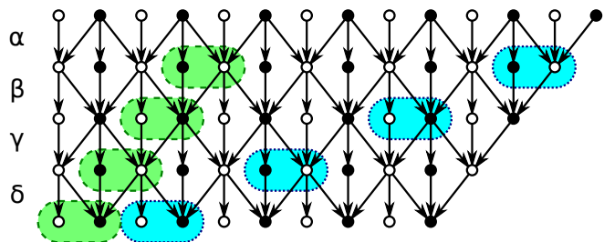
Fig. 1: Complete data flow graph of CDF 9/7 wavelet transform. The input signal is at the top, output at the bottom. The vertical (dashed) as well as the diagonal (dotted) vectorization are outlined.
