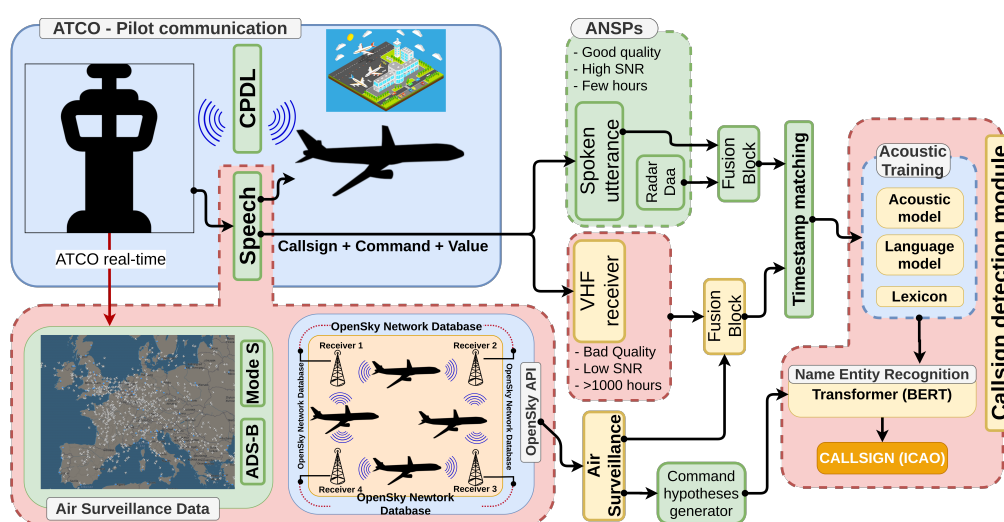
Figure 1. ATCO 2 proposed workflow for matching air surveillance data and spoken Air-Traffic Controller (ATCo)-pilot utterances gathered from the OpenSky Network API with speech data collected by VHF receivers. Each source (i.e., speech and air surveillance) is pre-processed before matching, e.g., speech data undergo voice activity detection and diarization. (i) Green blocks correspond to technologies either already on the market or available from previous projects, e.g., Active Listening Assistant (AcListant), MACHINE Learning Of speech Recognition models for Controller Assistance (MALORCA), Air-Navigation Service Providers (ANSPs), OSN, or earlier. (ii) Red blocks summarize the task/technologies that ATCO 2 is aiming to develop or improve.
