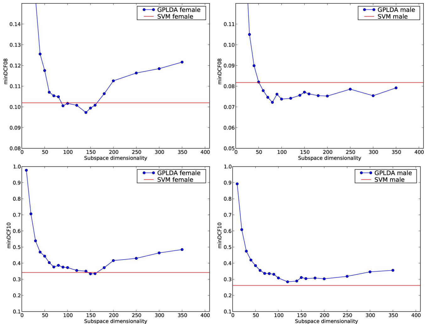
Fig. 1. minDFC08 and minDCF10 as a function of the speaker subspace dimensionality for the female and male speakers.
