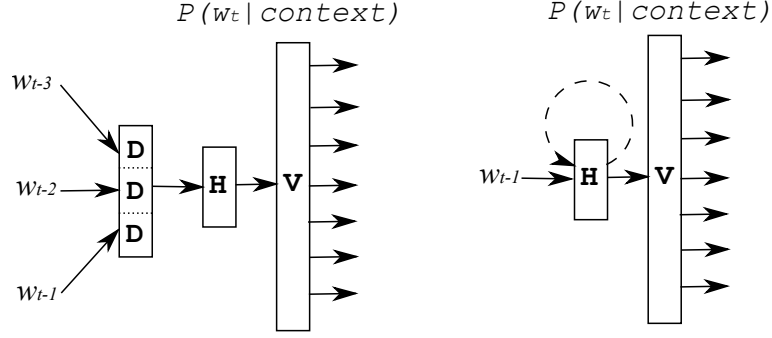
Figure 6.1: Feedforward neural network 4-gram model (on the left) and Recurrent neural network language model (on the right).
